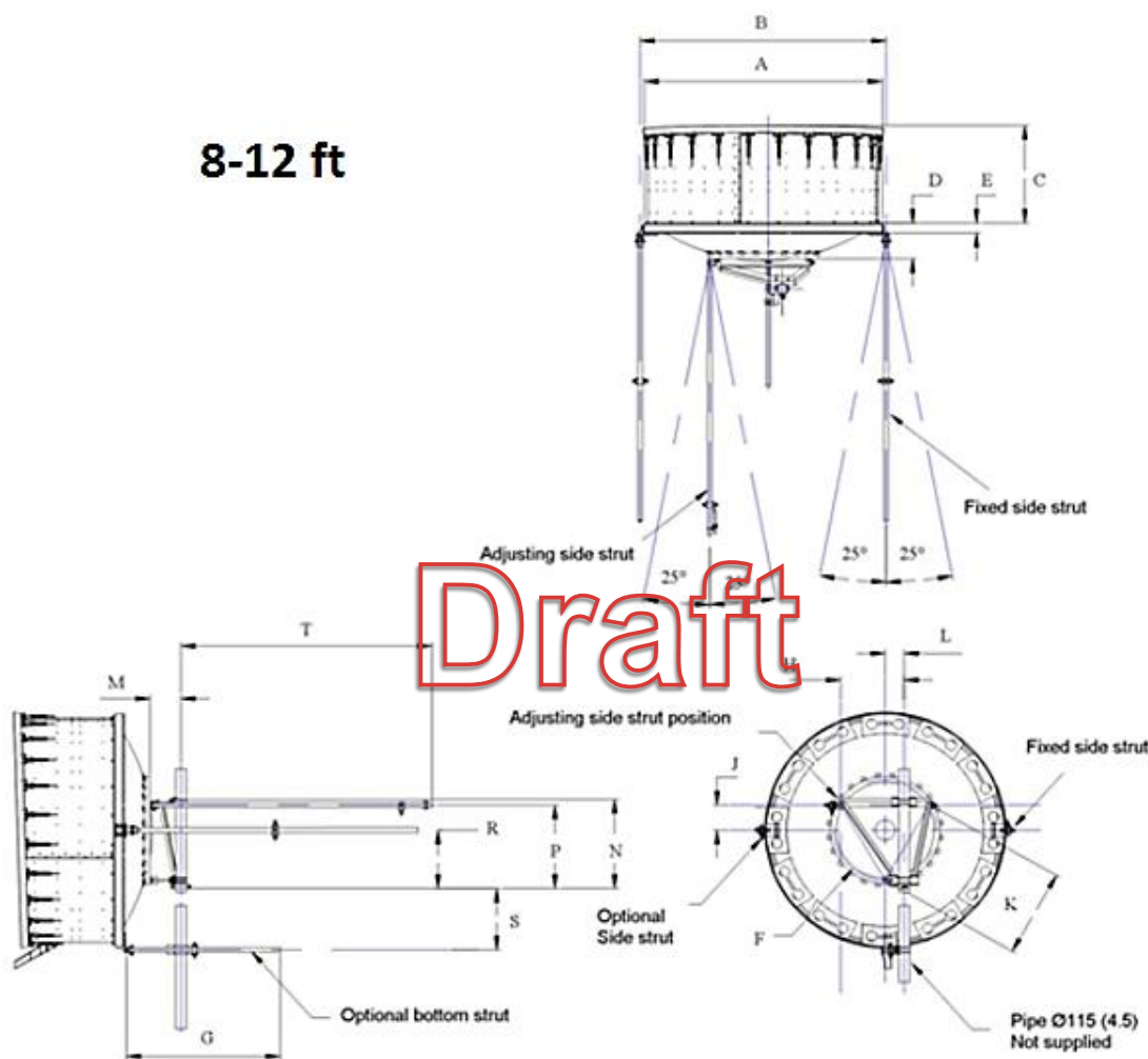
Antenna Dimensions (8-12 ft)
